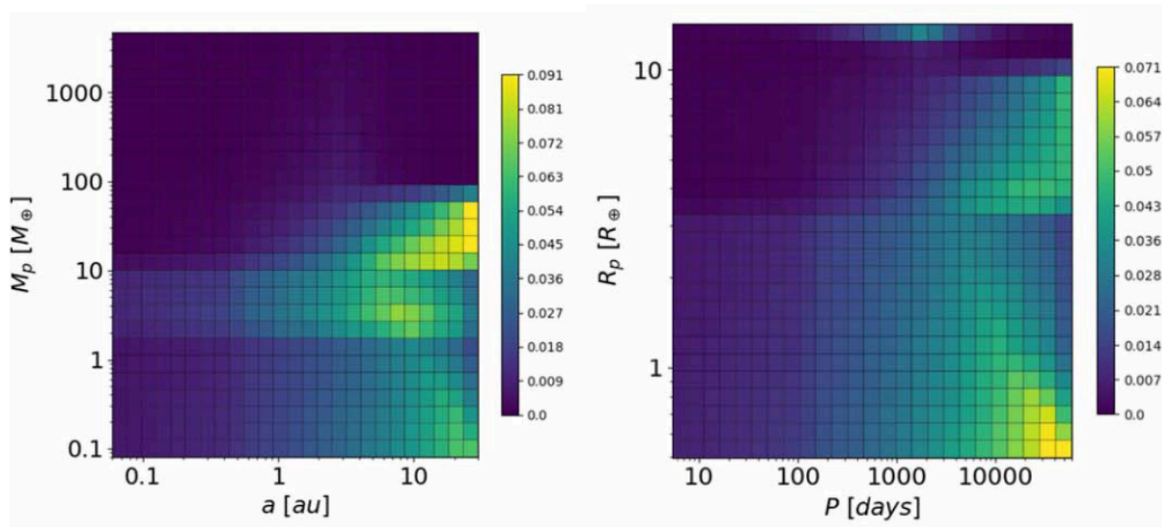
Figure 3: Default "Nominal" planet occurrence rates from Dulz et al. (2020).
