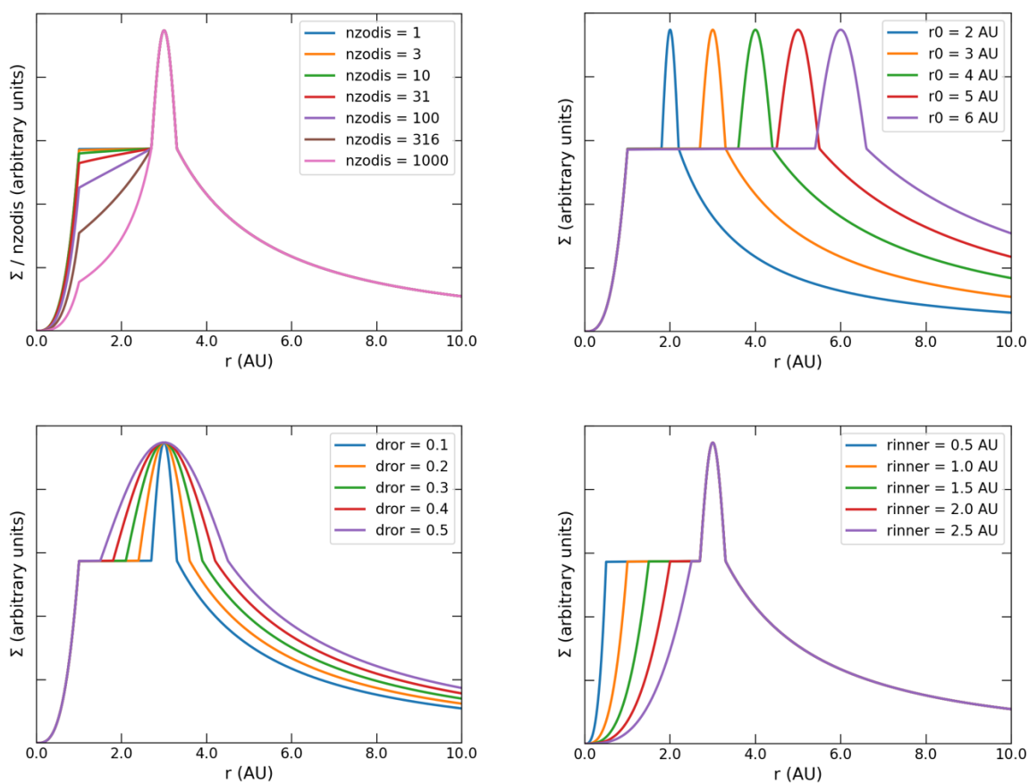
Figure 5: Example disk surface density profiles demonstrating the effect of the shape parameters.
