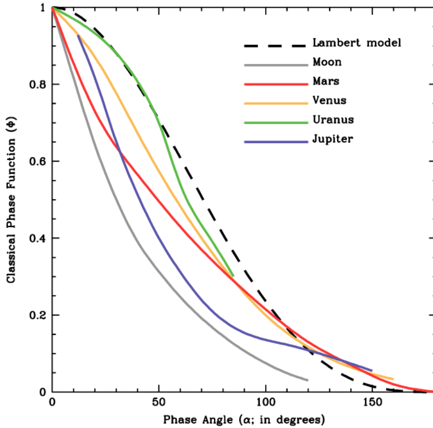
Figure 2: Phase curves of Solar system objects from Sudarsky et al. (2005), used for the default bounds in the phase function spread.
