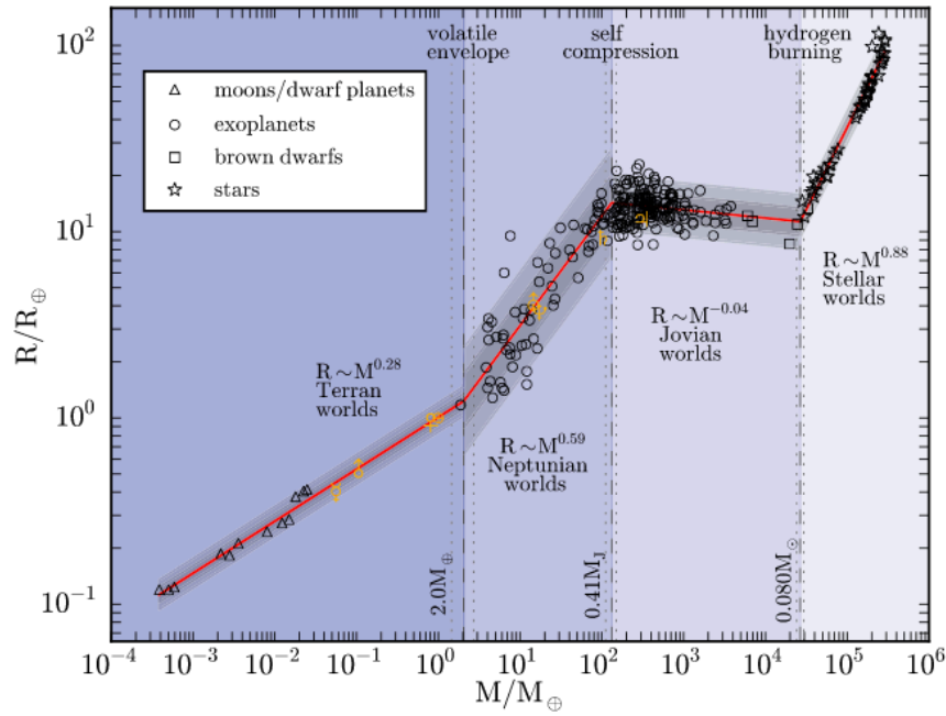
Figure 4: The default mass-radius relation from Chen & Kipping (2017).
