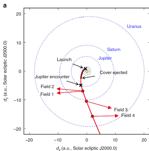
Figure 1 | The trajectory of New Horizons through the solar system. Data collection periods of relevance to this study are indicated. Both the x - y and r - z planes are shown ( a , b , respectively), with the axes in solar ecliptic units and d_r = \sqrt{d_x^2 + d_y^2} . New Horizons was launched from Earth at 1 a.u., and the data with the LORRI dust cover in place were acquired at 1.9 a.u., just beyond Mars' orbit at 1.5 a.u. (inner blue dotted lines). The dust cover was ejected near 3.6 a.u., and the data were acquired before and during an encounter with Jupiter. The data considered here were taken between 2007 and 2010 while New Horizons was in cruise phase. The red vectors indicate the relative positions of fields 1–4 compared to the sun and plane of the ecliptic.
