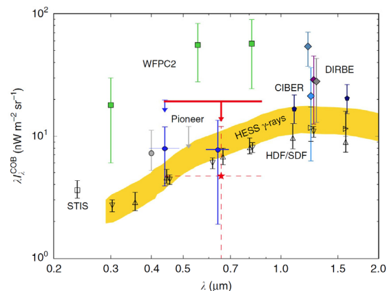
Figure 2 | Measurements of the COB surface brightness. The \lambda_{\lambda}^{\text{COB}} determined in this study are shown as both an upper limit (red) and a mean (red star). We also show previous results in the literature, including direct constraints on the COB (filled symbols) and the IGL (open symbols). The plotted LORRI errors are purely statistical and are calculated from the observed variance in the mean of individual 10 s exposures; see Fig. 3 for an assessment of the systematic uncertainties in the measurement.
