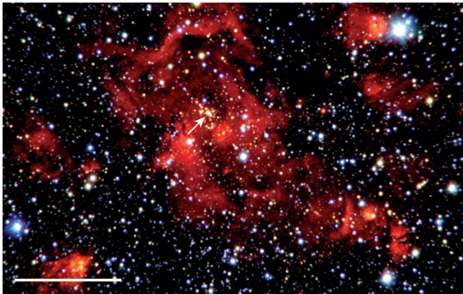
Figure 1 | Nestled in a young star cluster. The arrow indicates the location of W49nr1, a massive star identified by Wu et al. 1 in the central star cluster of the star-forming region W49. Scale bar, 1 arcminute.
