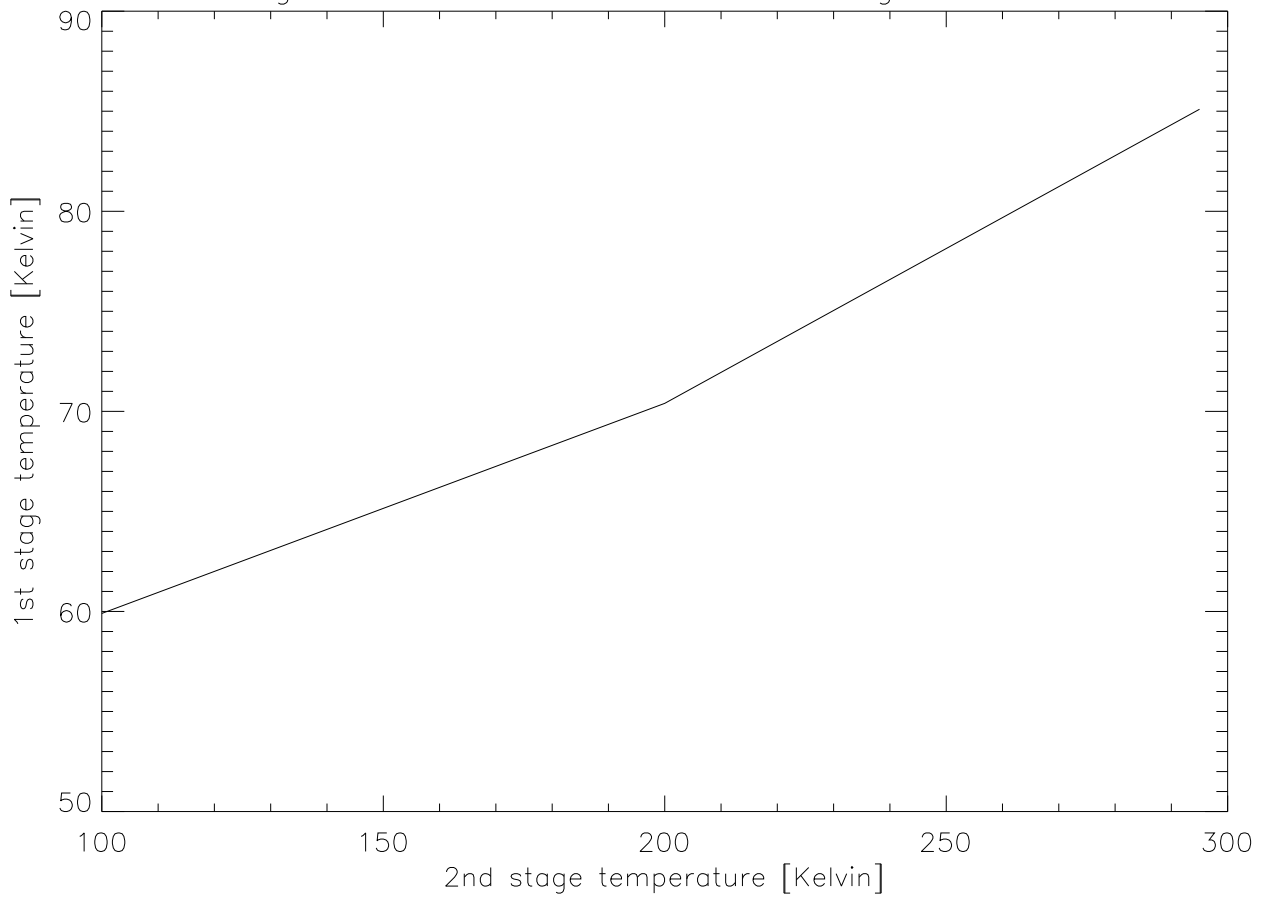
T: 1st stage near detector head vs 2nd stage at detector head
